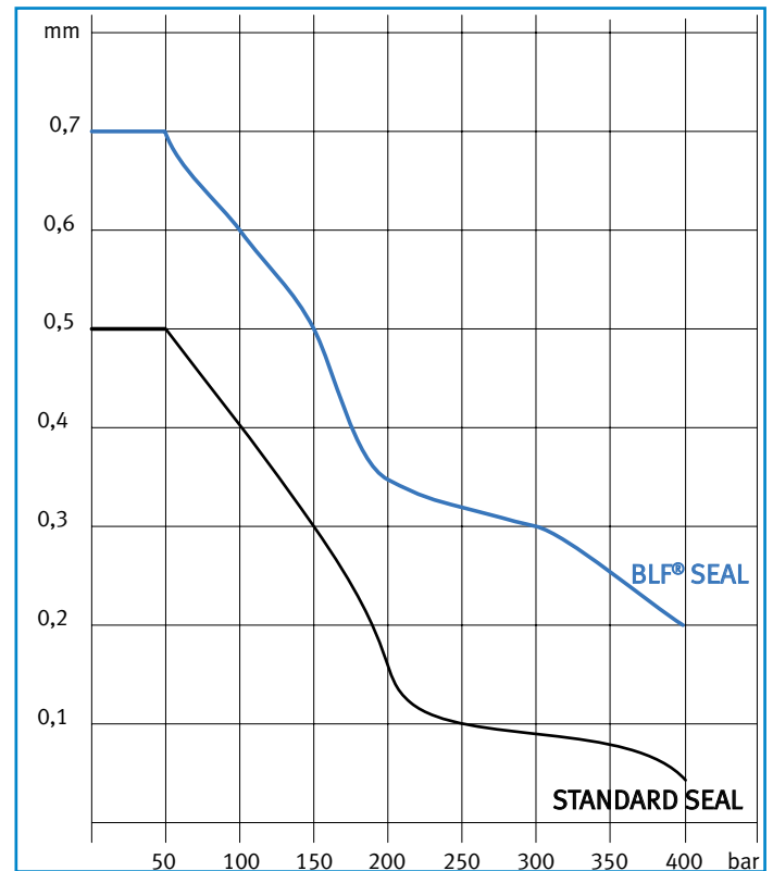
Fig. 30 - Pic.30: PRESSURE / COUPLING CLEARANCE
